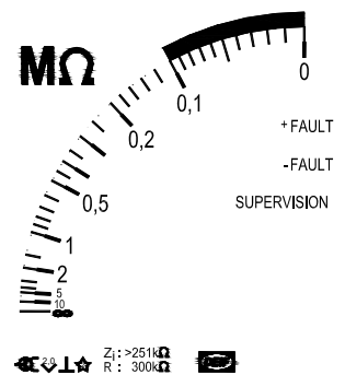
Fig. 2, 10...0MΩ scale
