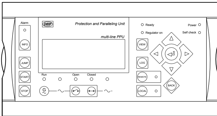
Display without Local control buttons (option Y11)
