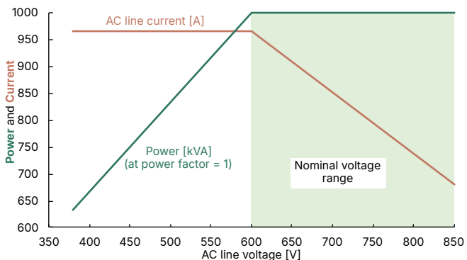
AC line voltage relative to the DC link
