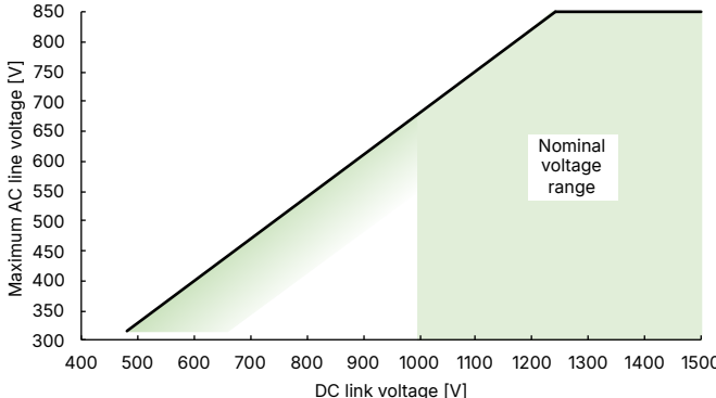
DC link voltage relative to the AC line
