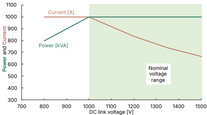
AC line power, current, and voltage curve
