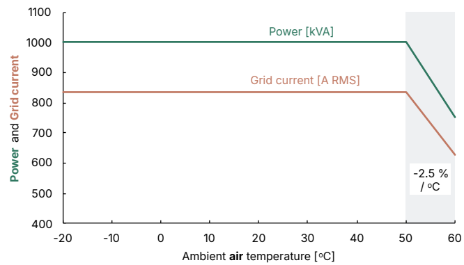
Ambient air (operating at 850 V AC)
