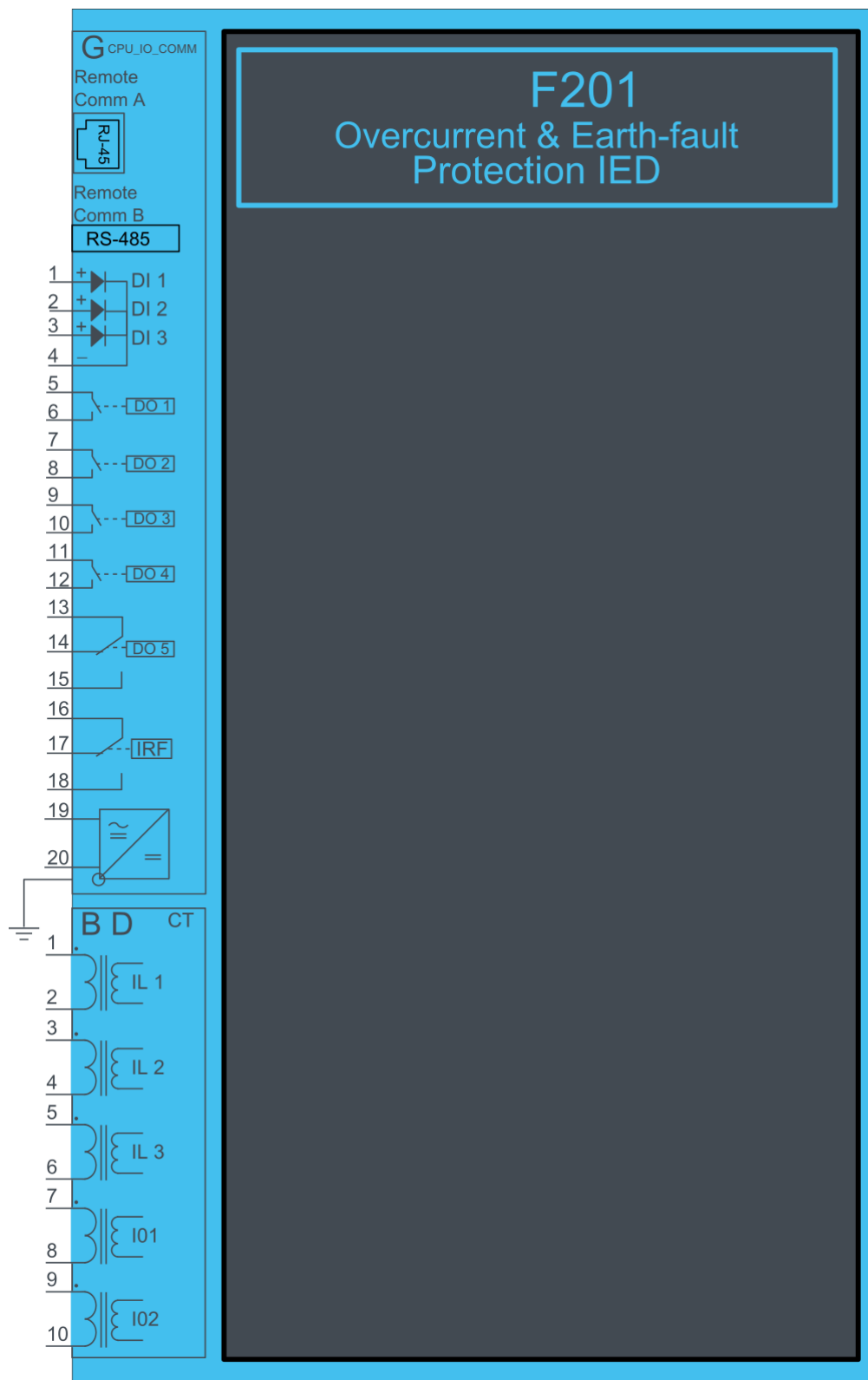
Figure 4.1 F201 hardware.
