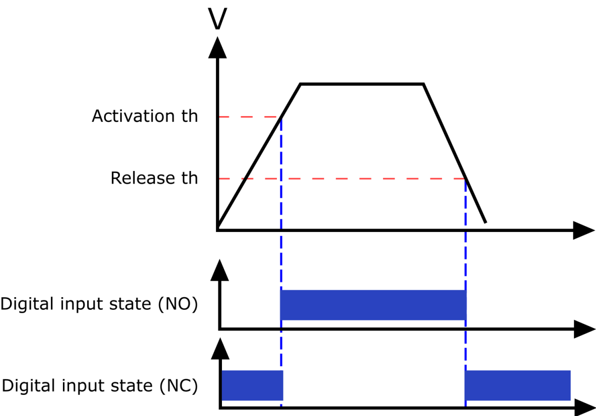
Figure 3.11 Digital input state when energizing and de-energizing the digital input channels.
