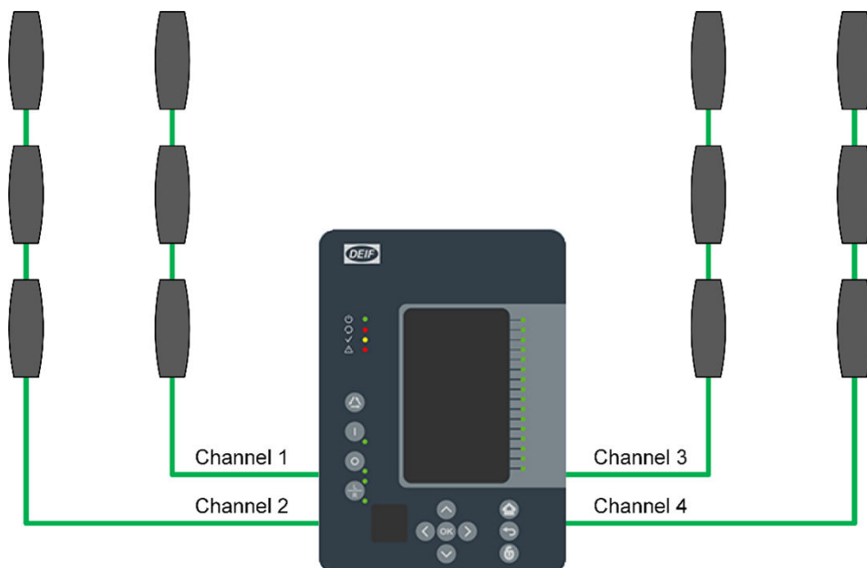
Figure 3.13 System overview
