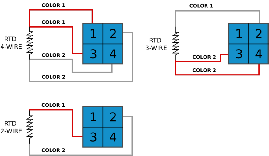
Figure 3.15 RTD sensor connection types.
