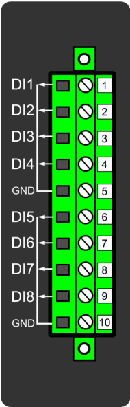
Figure 3.10 DI8 Binary input module with eight add-on binary inputs.
