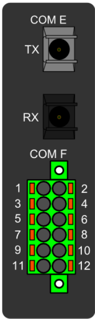
Figure 3.21 Serial RS232-card connectors
