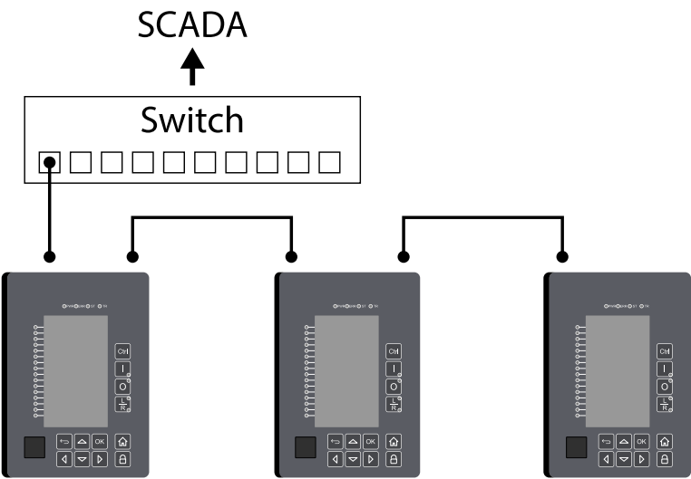
Figure 3.18 Example of a multidrop configuration.
