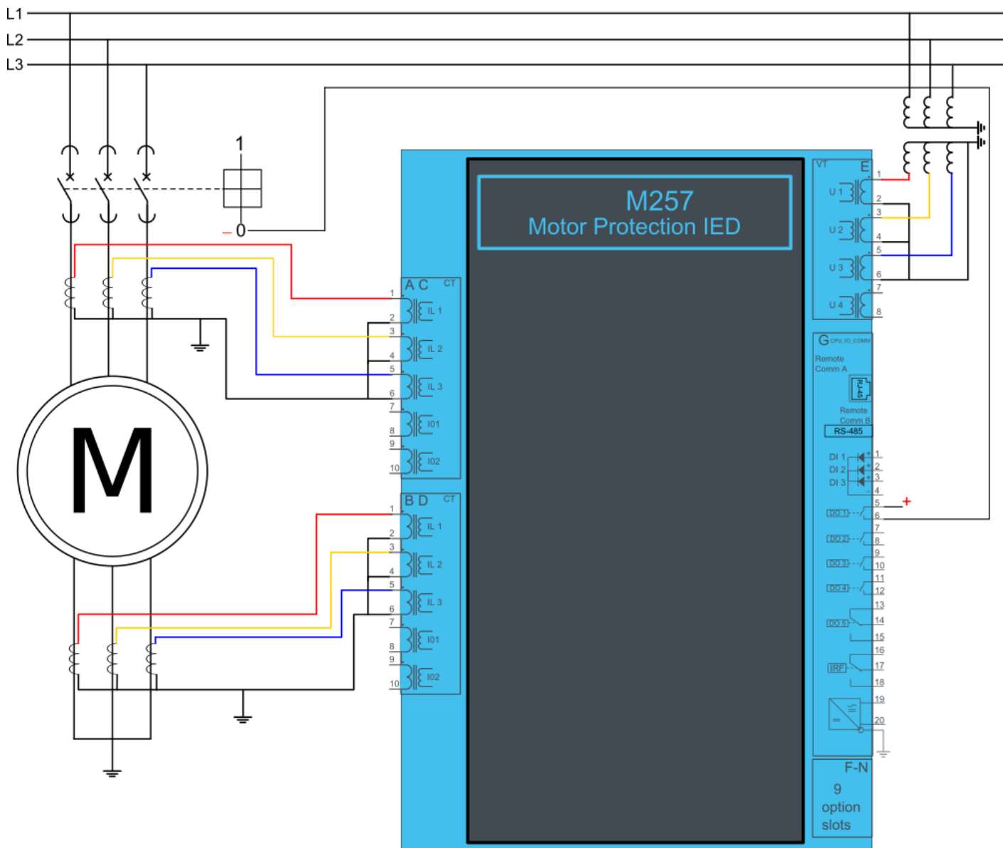
Figure 4.35 Example motor differential protection application drawing.
