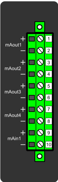
Figure 3.19 mA output & input module connections.
