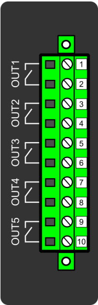
Figure 3.12 DO5 Binary output module with five add-on binary outputs.
