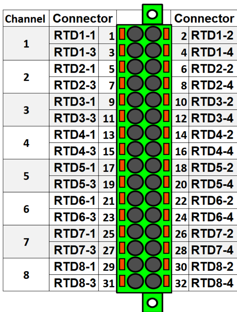
Figure 3.14 RTD input module connectors.
