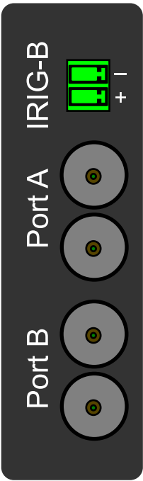
Figure 3.17 Double ST 100 Mbps Ethernet communication module connectors.
