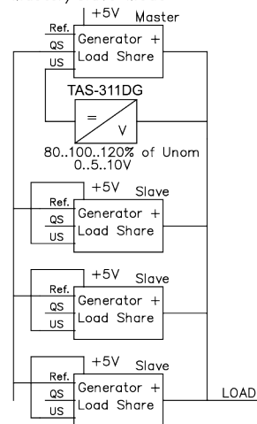
Master/Slave Mode
