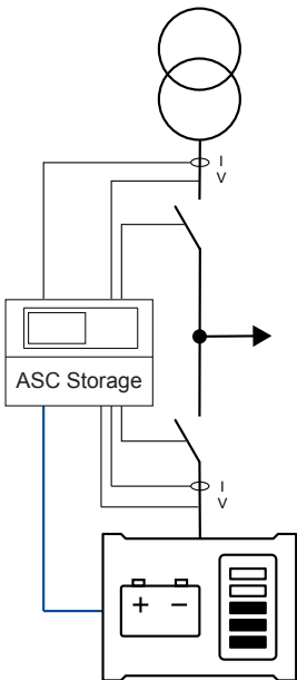
Peak shaving application
