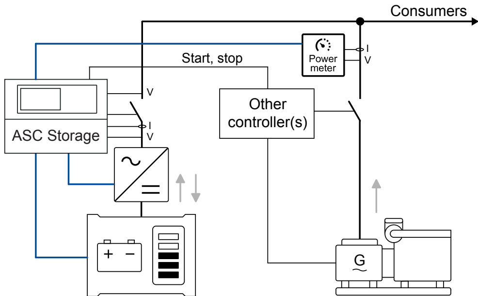
Emission-free power rental solution with a single ESS
