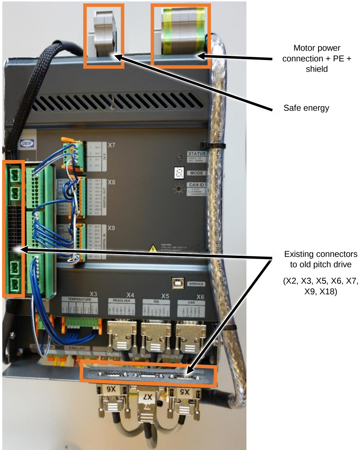
Figure 1 IMD 100 with wire harness connections overview
