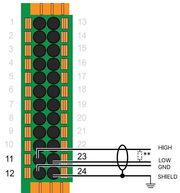
CAN port 2**
