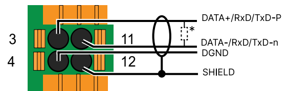
Profibus Master port 2
