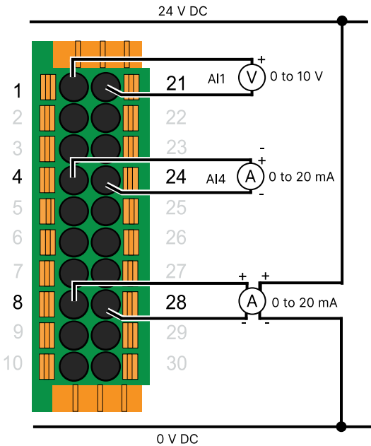
Active transducer
