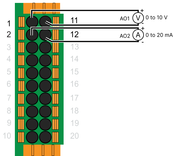
Analogue outputs
