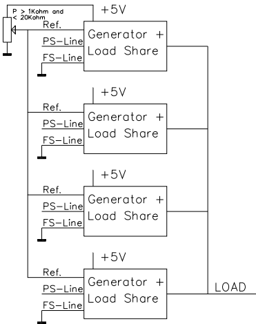
Fixed load to busbar – No frequency control
