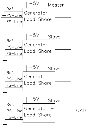
Master/Slave Mode
