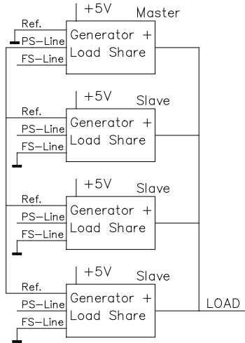
Master/Slave Mode
