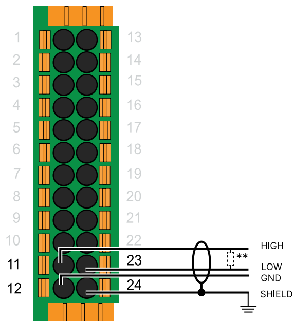
CAN porta 2**
