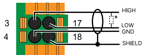
CAN porta 2
