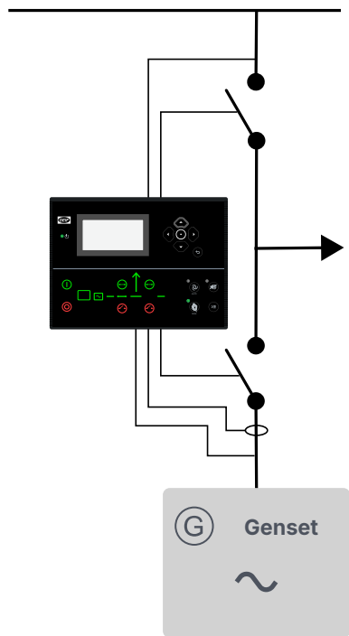
Emergency genset
