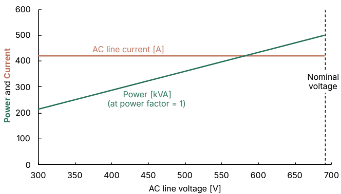
AC line voltage relative to the DC link
