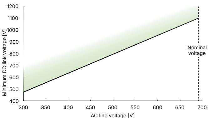
DC link voltage relative to the AC line
