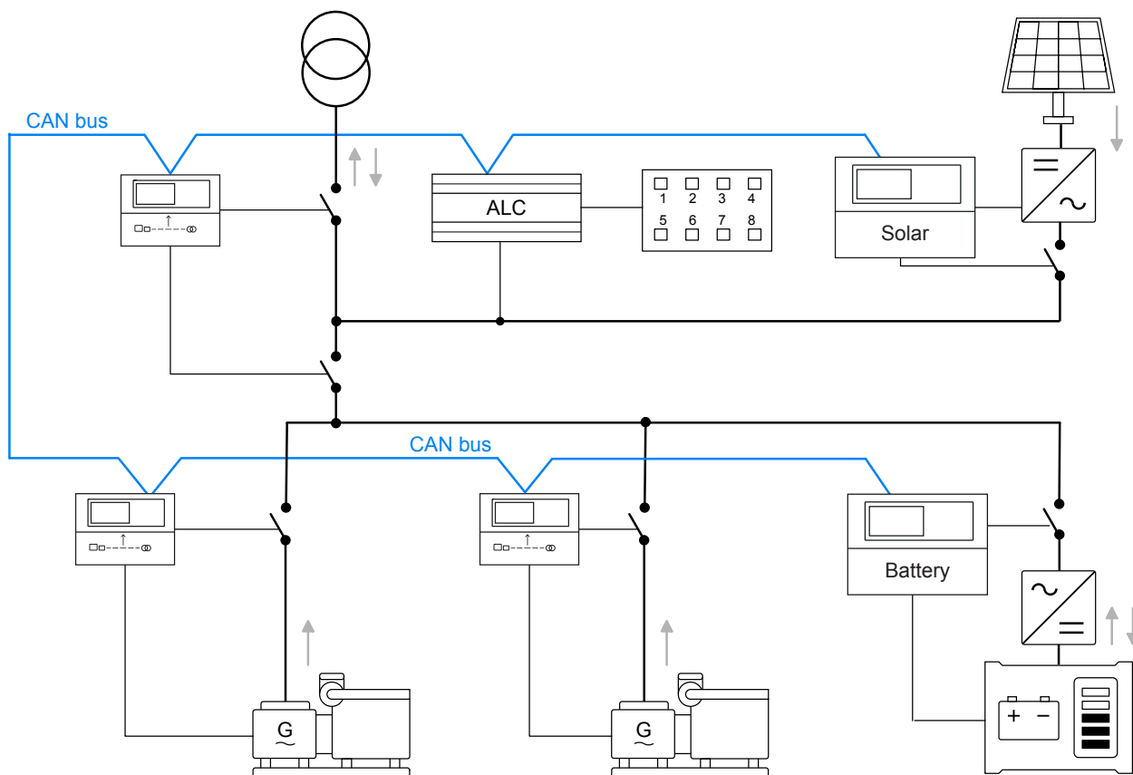
iE 150 in power management with battery and solar controllers
