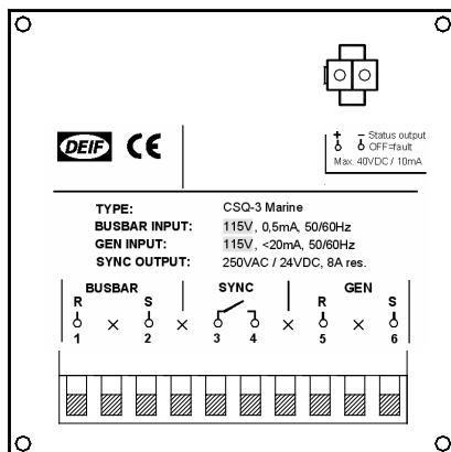
Version marine
